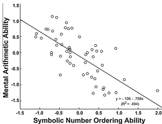
Fig. 2. Scatterplot of the relation between symbolic number-ordering ability and complex mental-arithmetic ability. Note that higher numbers indicate worse performance for numeral-ordering, but better performance for complex mental-arithmetic.
